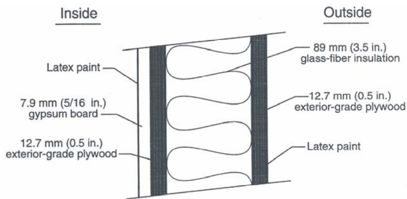
Variable - Permeance - Claddings Wall
