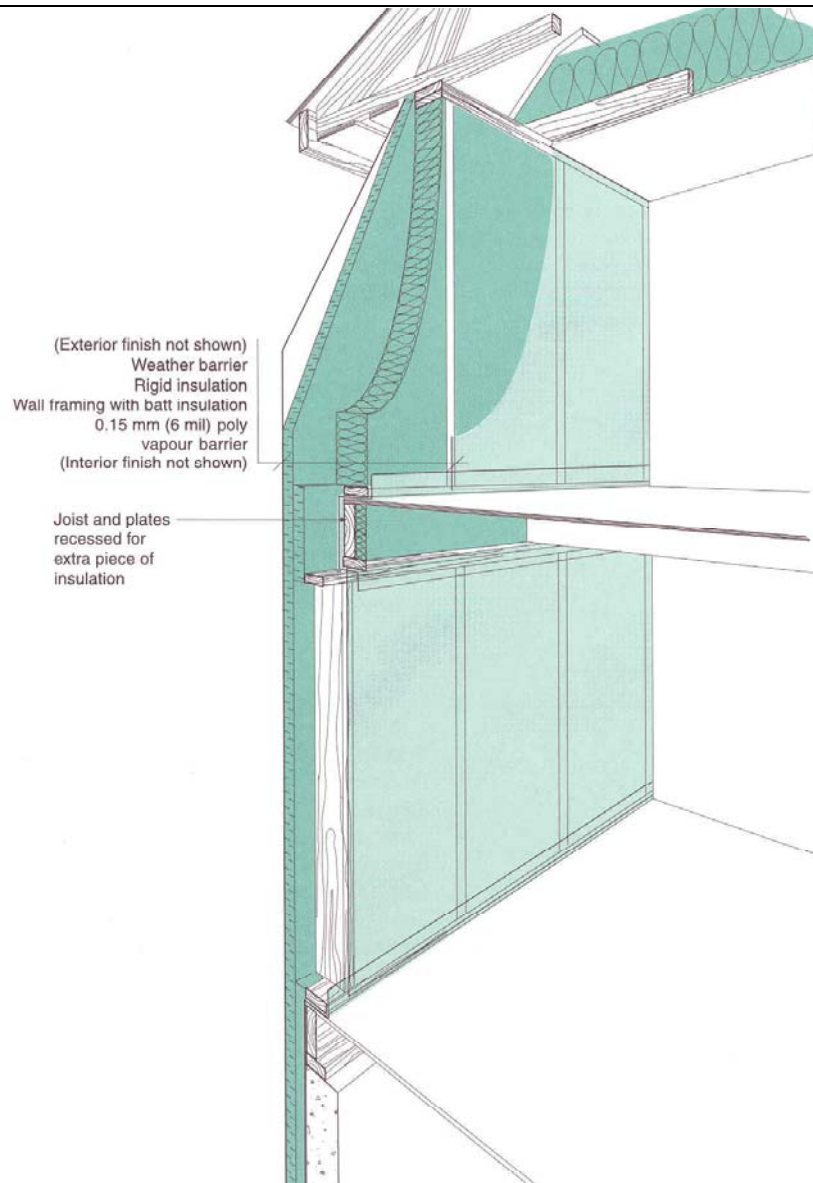
Single stud wall with exterior insulating sheathing
