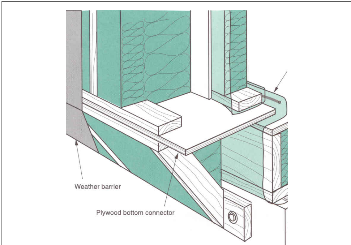
Foundation wall/floor/wall junction of a double stud walls system.
