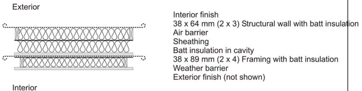
Figure 3. Double Stud Walls Assembly
