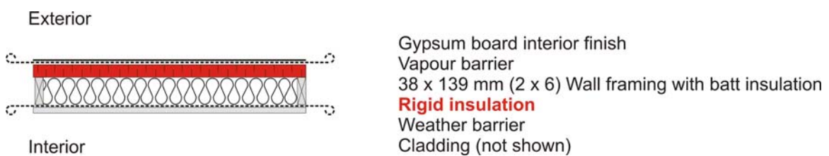
Figure 2. Thermally Upgraded Single Stud Wall
