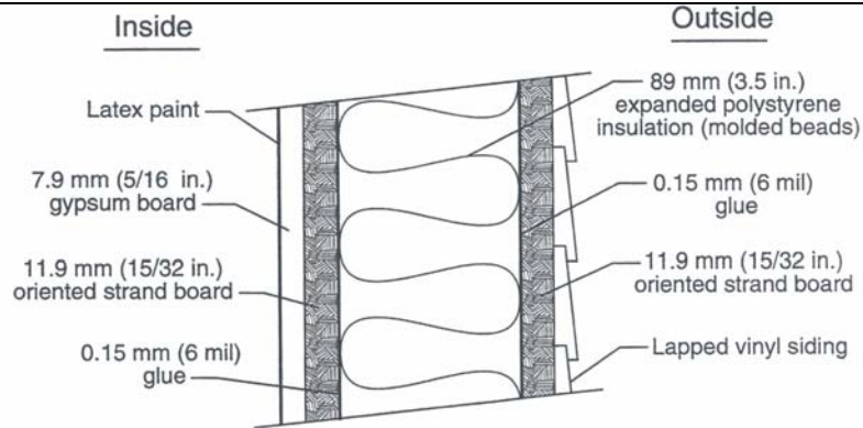
Sandwich panel wall with low-permeability insulation
